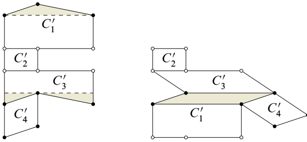
Figure 23: Deformation of a surface in Case 4.II.OA to Case 4.II.OC
