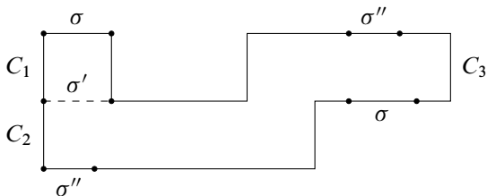
Figure 12: Cylinders in Proposition 5.6, Case 2
