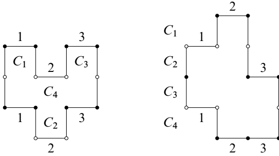
Figure 20: \mathcal{H}^{\text{odd}}(2, 2) , Cases 4.I.OA (left) and 4.I.OB (right)
