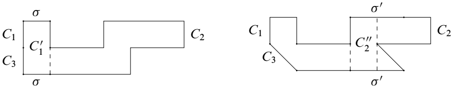
Figure 11: Cylinders in Proposition 5.6, Case 1
