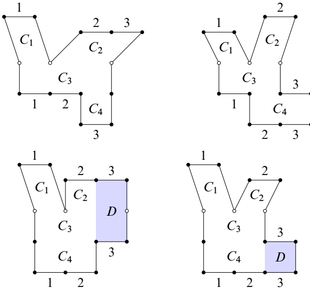
Figure 16: 4–cylinder diagrams in \mathcal{H}(3, 1) , Cases 4.III.UA (top left), 4.III.UB (top right), 4.III.UC (bottom left) and 4.III.UD (bottom right)
