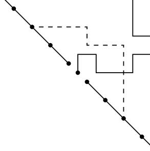
Figure 1: The diagonal lines D^+ (top left) and D^- (bottom right), a directed dual path (dashed) in H from D^+ to D^- , and a primal path (solid) in H^+ from the origin (centre).
