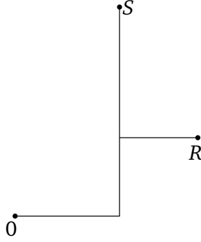
Figure 2: The subgraph \pi connecting 0 to R and to S.
