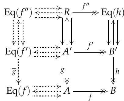
Figure 2: Closedness of \mathcal{S} -special regular epimorphisms under coequalisers of certain reflexive graphs
