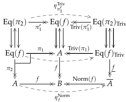
Figure 1: The construction of \text{Norm}(f)
