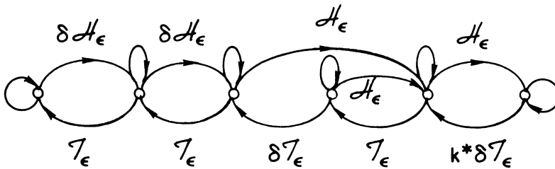
FIG. 2. An alternative \epsilon -optimal algorithm.
