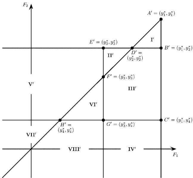
FIG. 3. Regions of the set D .
