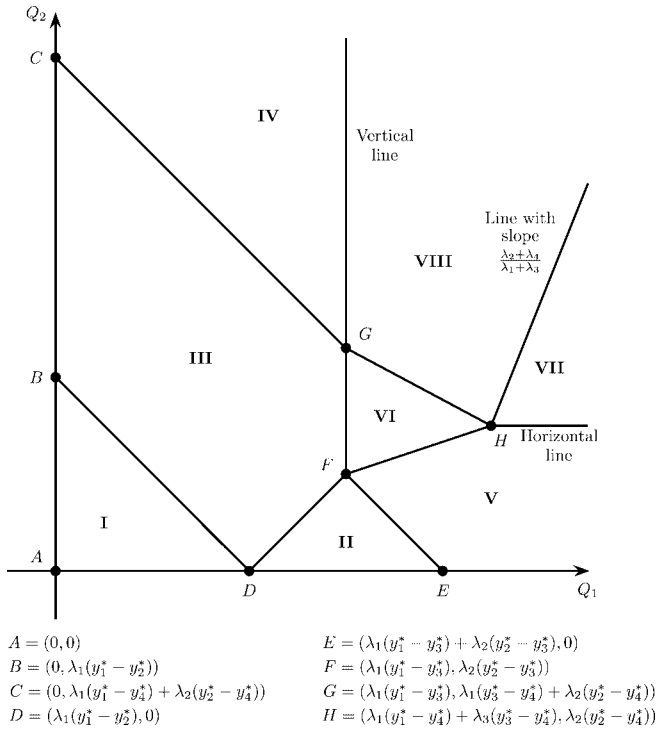
FIG. 2. Regions of the set [0, \infty)^2 .
