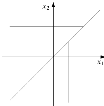
Figure 1: Two examples of equivalence classes for the relation defining the quotient module B : \{x^2 = 2, x^1 < 2\} and \{x^1 = 1, x^2 \leq x^1\}
