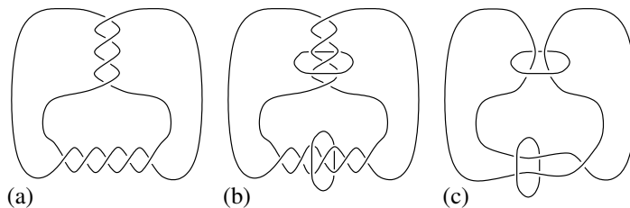
Figure 2: (a) The original link diagram K (b) Crossing circles added (c) The diagram of L
