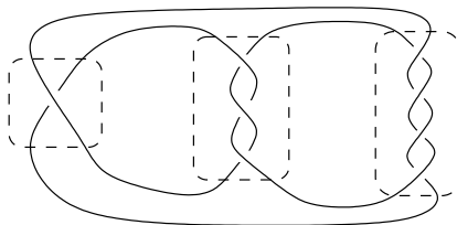
Figure 1: Twist regions of the diagram are encircled with dashed lines. For this diagram, \text{tw}(D_K) = 3 .
