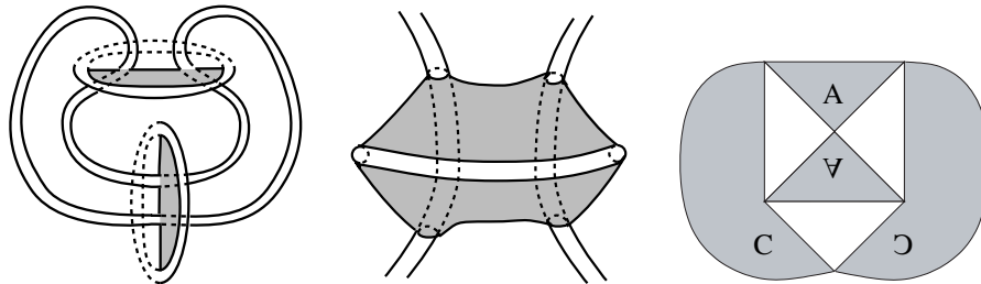
Figure 3: Decomposing S^3 - L into ideal polyhedra: first slice along the projection plane, then split the remaining halves of two-punctured disks to obtain the polyhedron on the right.
