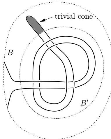
Figure 1: A graph which is knotted in a ball because of a trivial cone
