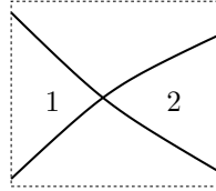
Figure 4: A crossing at which l_c switches, without implying that \Sigma is weakly reducible
