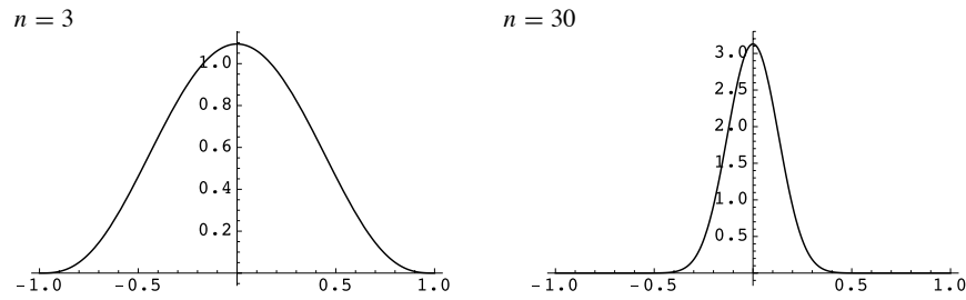
FIGURE 1.1. Approximate identity. Graphs of c_n(1-x^2)^n for n = 3 and n = 30 with different scales used on the vertical axes.
