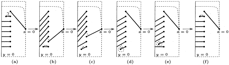
Fig. 12. The move of intervals on H_\theta in the case q = 2 . The figures are in the case p = 8 .
