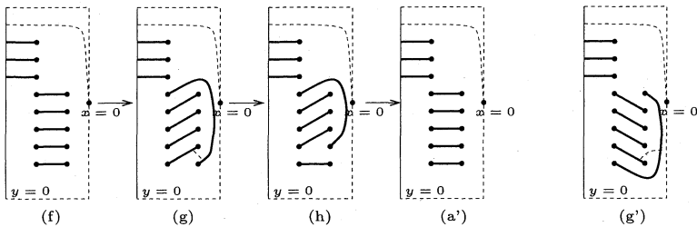
Fig. 8. The move of intervals during the 1/r -rotation of L_{\bar{g}} \cap H_\theta in case (A-1).
