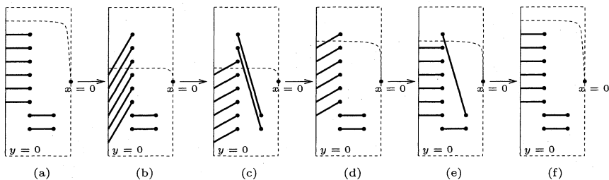
Fig. 10. The move of intervals on H_\theta in case (A-2).
