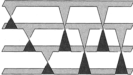
Fig. 1. An example of quasipositive surface.
