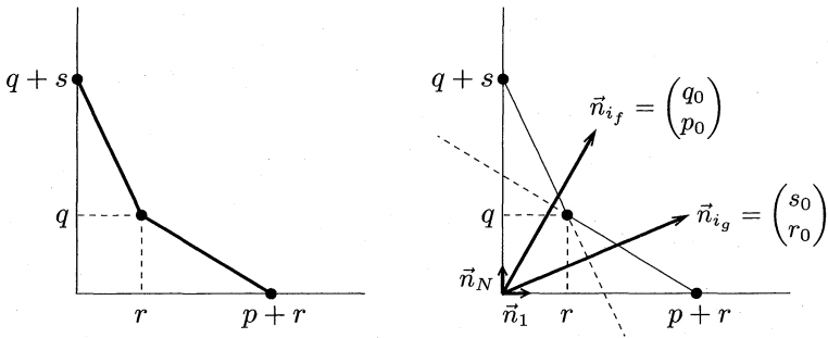
Fig. 2. The Newton boundary of (fg, O) in the case p/q > r/s .
