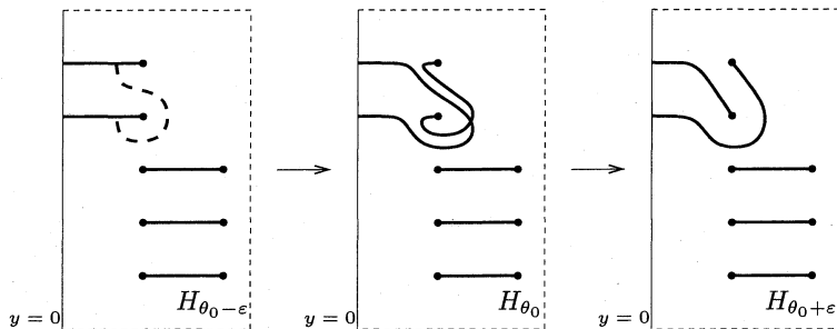
Fig. 5. An example of a saddle appearing in the move of S \cap H_\theta .
