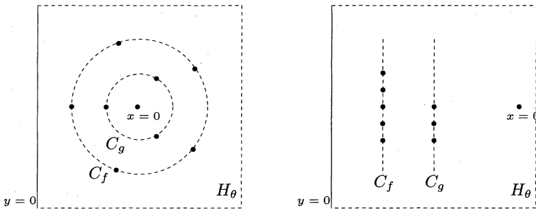
Fig. 4. The intersection points of L_f and L_g with H_\theta . The figures are in the case p = 5 and r = 3 .
