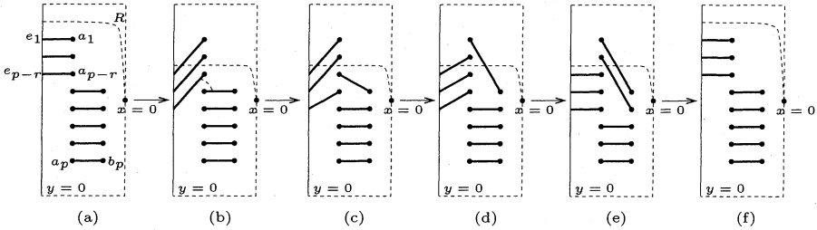
Fig. 6. The move of intervals on H_\theta in case (A-1) with q \leq p - r .
