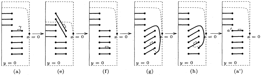
Fig. 9. The simple closed curve \gamma on S in the case s > q .
