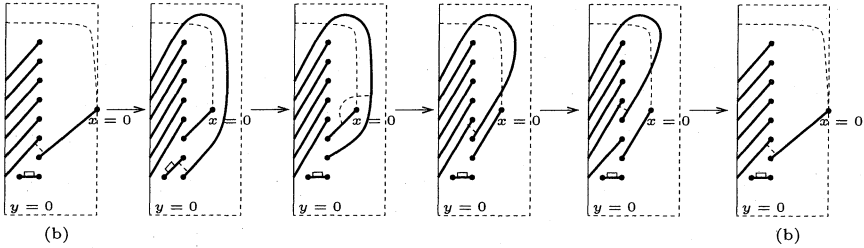
Fig. 13. The additional move of the intervals on H_\theta in the case q > 2 . The figures are in the case p = 8 .
