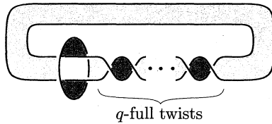
Fig. 14. The fibre surface in the case p = 1 and q \geq 1 .
