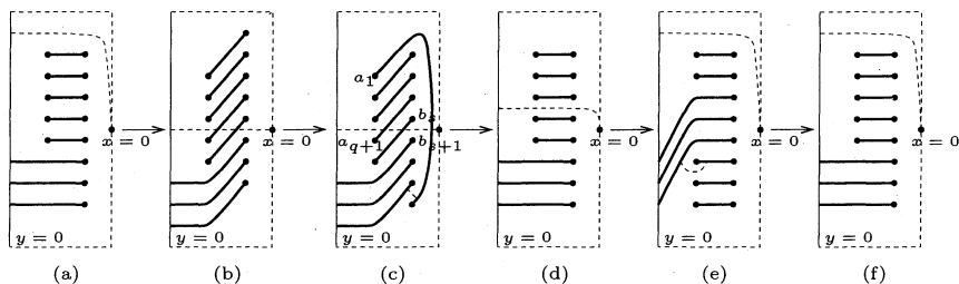
Fig. 11. The move of intervals on H_\theta in case (B).
