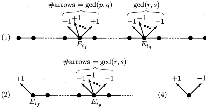
Fig. 3. The dual resolution graphs in cases (1), (2) and (4).
