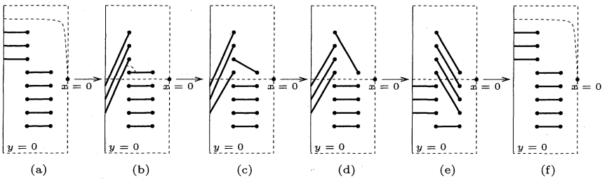
Fig. 7. The move of intervals on H_\theta in case (A-1) with q > p - r .
