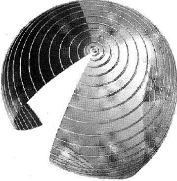
Fig. 6. A branched Bonnet surface of type \mathbf{B}
