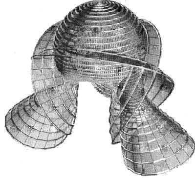
Fig. 7. Bonnet surface of type \mathbf{B}_\nu
