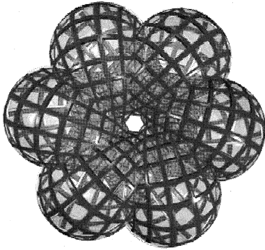
Fig. 2. Twisted Wente torus
