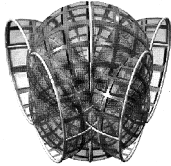
Fig. 3. One fundamental piece of a torus with spherical curvature lines
