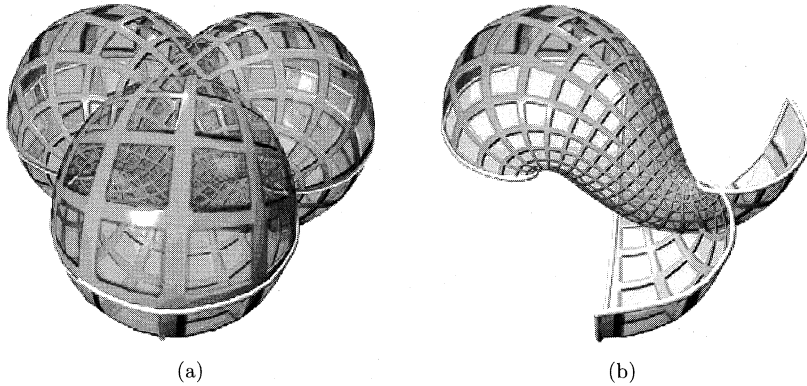
Fig. 1. Wente torus having a threefold symmetry, and one fundamental piece
