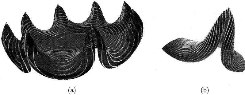
Fig. 8. Bonnet disk with a critical point with J = 6 , and its cusp
