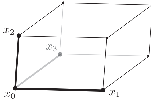
(a) The induced parallelotope and normalizing edges for computing p_2 \sin_{x_0}(X)
