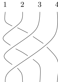
FIGURE 1: The Garside element \Delta \in B_4^+ .
