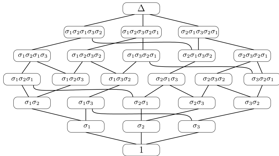
FIGURE 2: The lattice of simple elements in B_4^+ .
