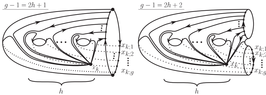
FIG. 10. N_{g-1}^{(k)} is diffeomorphic to the surface on the left-hand side (resp. right-hand side) of the figure when g - 1 = 2h + 1 (resp. g - 1 = 2h + 2 ). We regard the above surface on the left-hand side as the surface identified antipodal points of the boundary component, and the above surface on the right-hand side as the surface attached their boundary components along the orientation of the boundary.
