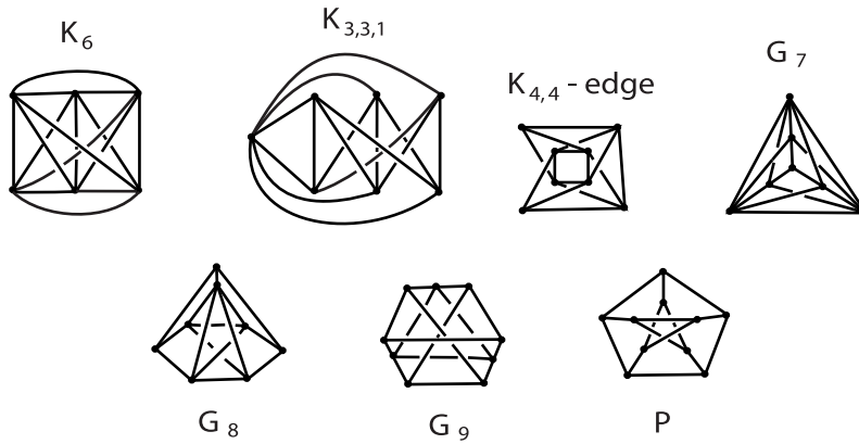
Fig. 1. The Petersen family of graphs.
