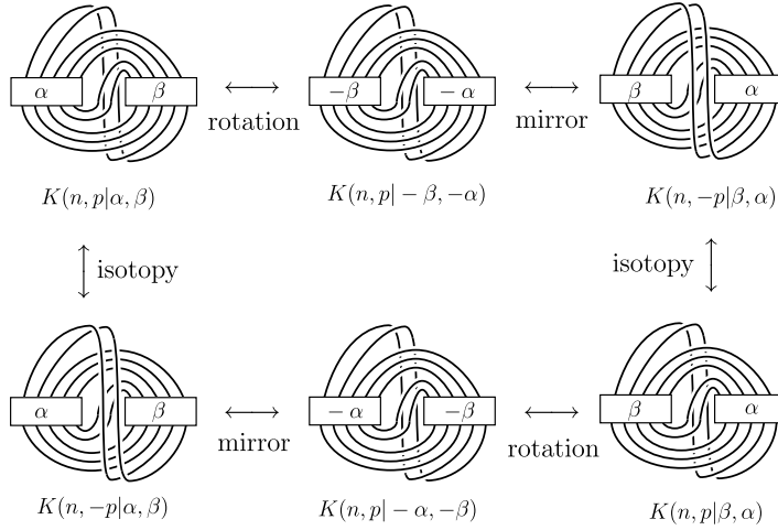
Fig. 3.3. Deformation of K(5, 2 | \alpha, \beta) .
