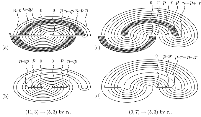
Fig. 7.1. Reductions by \tau_1 and \tau_2 .
