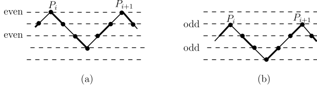
Fig. 8.1. Thick edges indicate odd edges.
