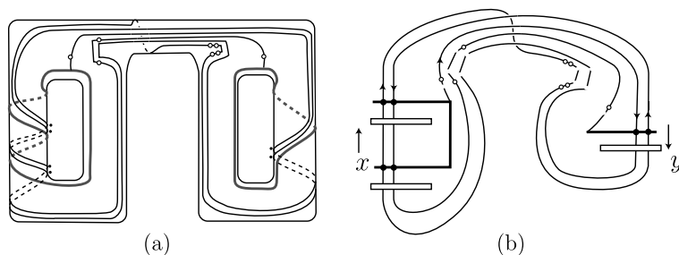
Fig. 13.4. K = K(5, 2 | 2, 1) , \tilde{W}(K) = yx^2y^{-1}x^{-2} , W(K) = xy \cdot 1 \cdot x^2y^2 \cdot y^{-3}x^{-3} \cdot xy .
