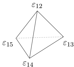
Figure 2: Three dimensional faces of \Delta .
