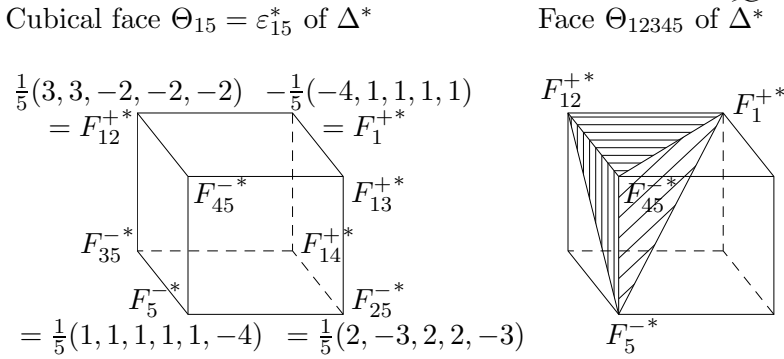
Figure 3: Three dimensional faces of \Delta^* and \widetilde{\Delta}^* .
