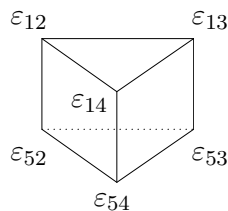
Figure 2: Three dimensional faces of \Delta .
