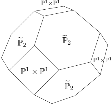
Figure 4: The threefold \overline{T_{F_i^{\epsilon^*}}} in \tilde{P} \setminus T .
