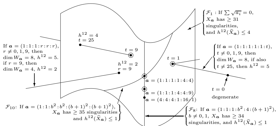
Figure 1: Values of the parameter \mathbf{a} for certain members and subfamilies of the family of Calabi-Yau threefolds X_{\mathbf{a}} , with \mathbf{a} for modular X_{\mathbf{a}} marked by a point, which is circled if X_{\mathbf{a}} is rigid.
