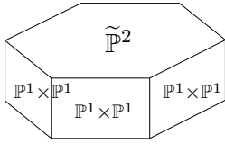
Figure 5: The threefold \overline{T_{F_{ij}^{\epsilon^*}}} in \tilde{P} \setminus T .
