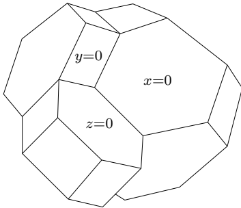
Figure 6: How \overline{\{x = 0\}} , \overline{\{y = 0\}} and \overline{\{z = 0\}} \subset \tilde{P} \setminus T meet.
