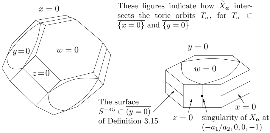
Figure 7: How \tilde{X}_a intersects P \setminus T .
