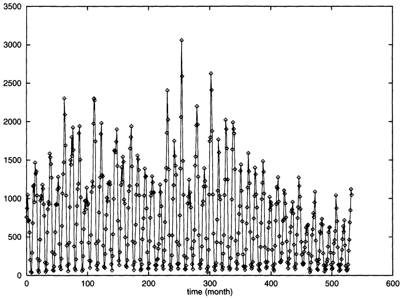
Figure 6: Data of chickenpox
