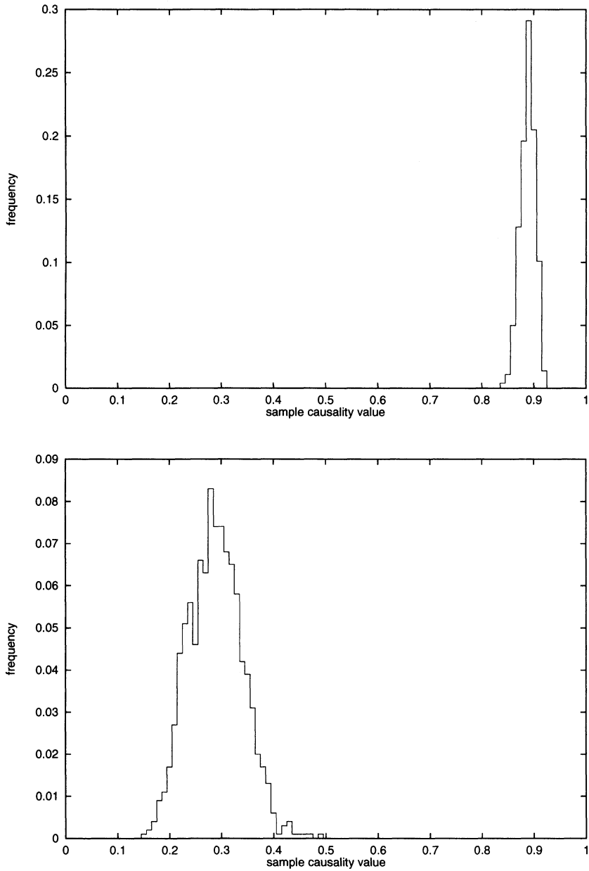
Figure 4: The distribution of the bootstrapped sample causality values (Top) and that of sample causality value between measles data and random sequences (Bottom): (II)
