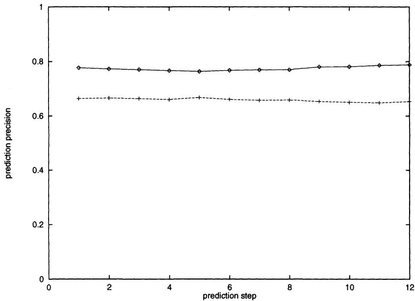
Figure 9: Prediction precision for chickenpox data. The solid line means correlation, and the dashed line means mean square root error.
