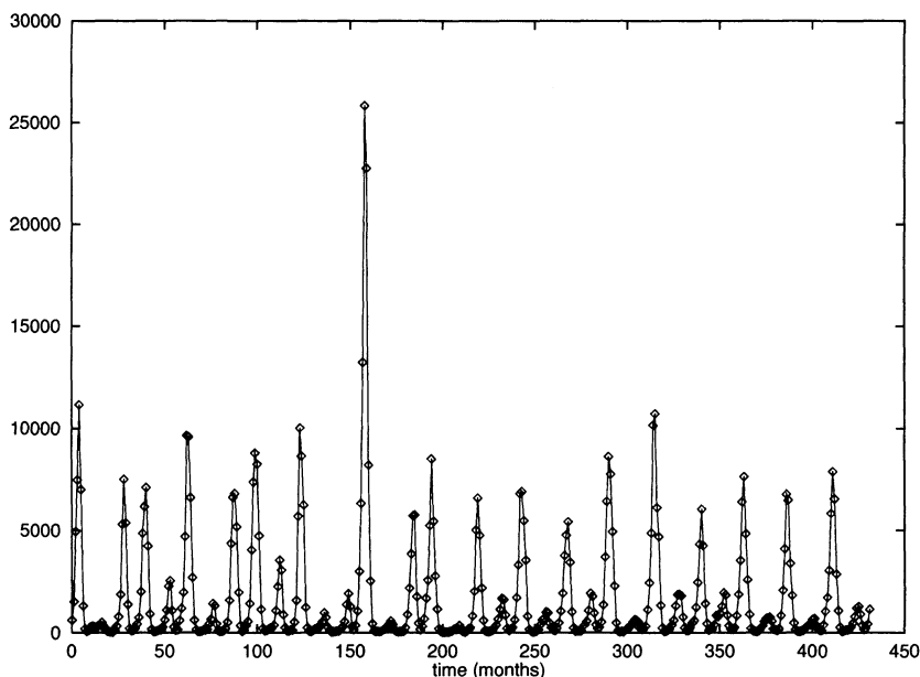
Figure 1: Data of measles
