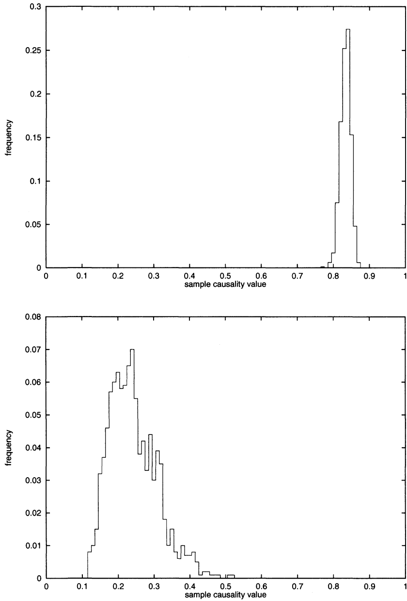
Figure 8: The distribution of the bootstrapped sample causality values (Top) and that of sample causality value between chickenpox data and random sequences (Bottom)
