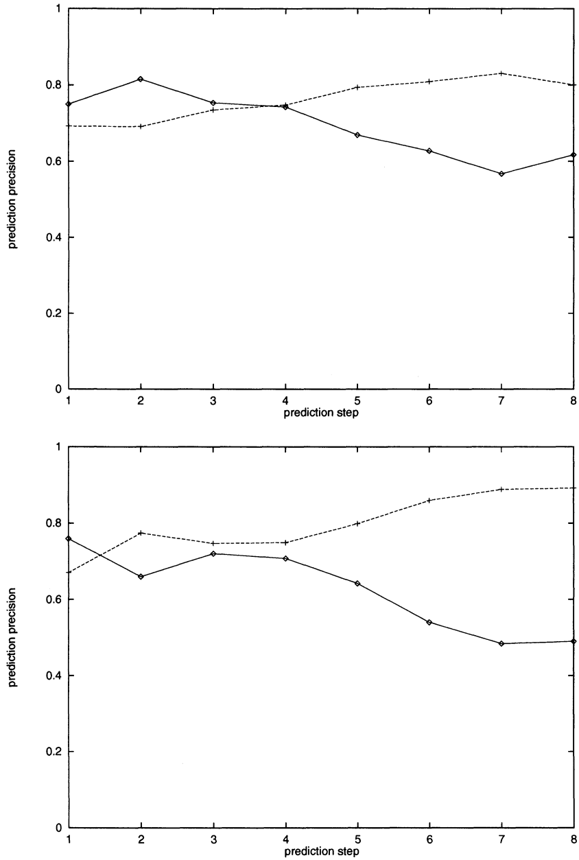
Figure 5: Prediction precision for measles data (I) (Top) and (II) (Bottom). The solid line and the dashed line stand for C(T) and E(T) , respectively.
