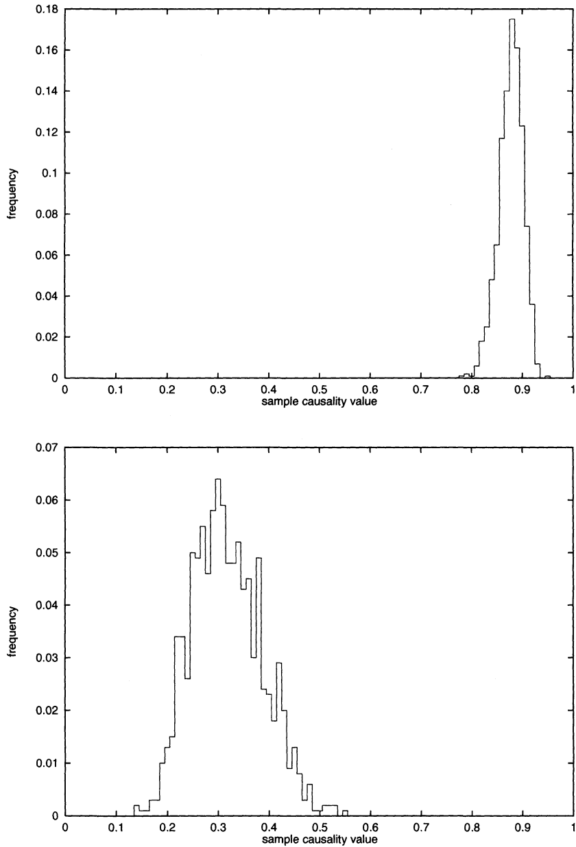
Figure 3: The distribution of the bootstrapped sample causality values (Top) and that of sample causality value between measles data and random sequences (Bottom): (I)
