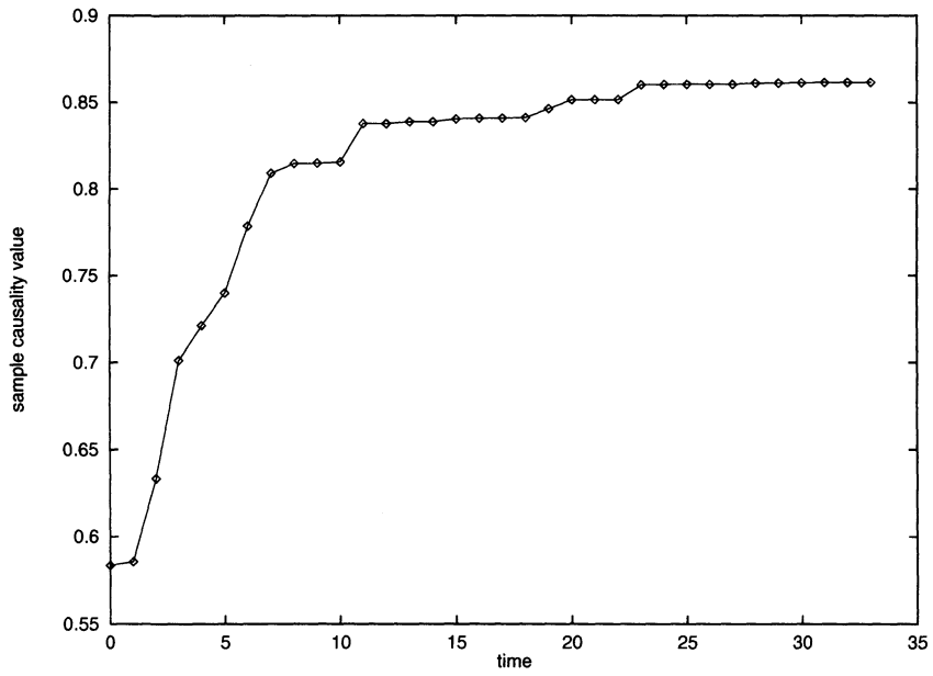
Figure 7: Sample causality function for chickenpox data
