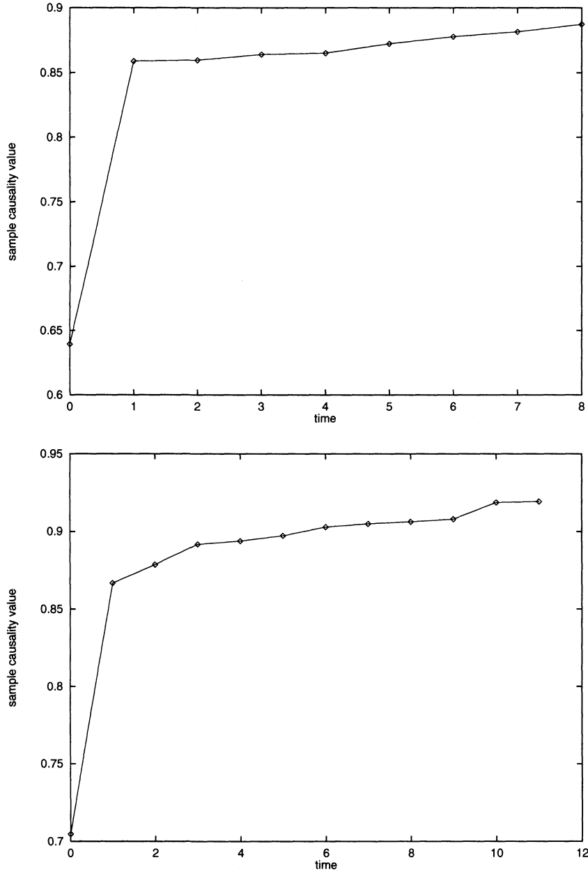
Figure 2: Sample causality functions for measles data (I) (Top) and (II) (Bottom)
