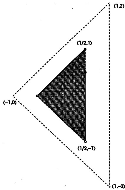
Figure 2: The sets \mathcal{D}_2^0 and \mathcal{E}_2 .
