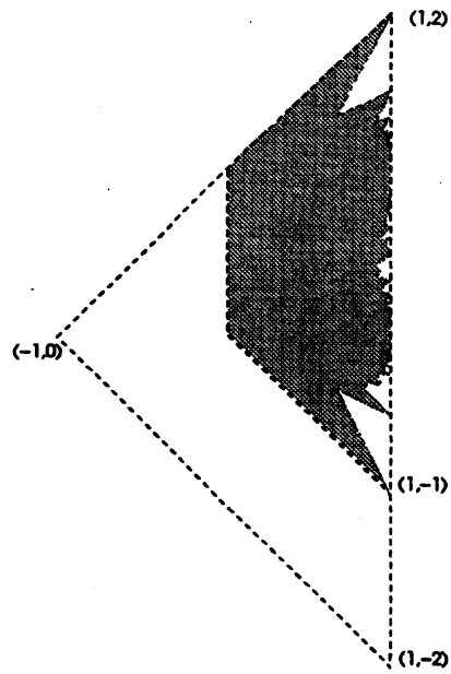
Figure 1: The sets \mathcal{D}_2^0 and \mathcal{E}_2 .
