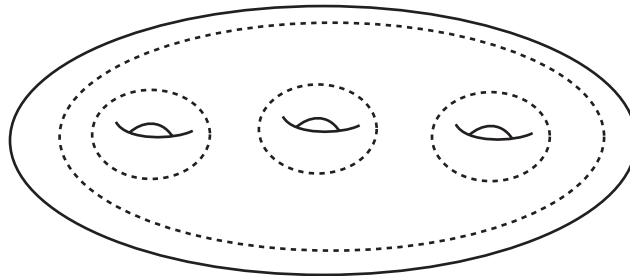
Figure 2. The collection of curves \Gamma is diffeomorphic to the collection of curves shown above.
