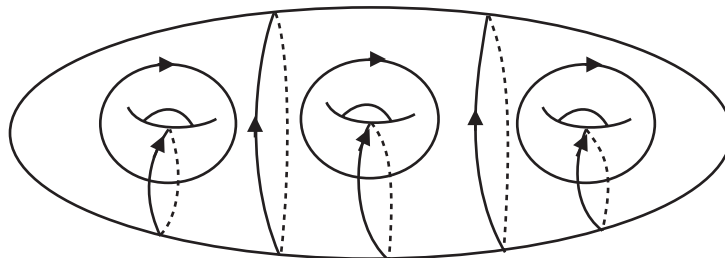
Figure 1. For 1 \leq i \leq 3 , let the \alpha_i be the half-hidden, non-separating, simple, closed curves and let \beta_i be the nonseparating curves such that \alpha_i \cdot \beta_i = 1 (with subscript increasing from left to right). Let the \lambda_j be the two separating curves again labeled left to right.
