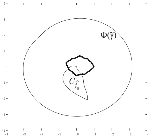
FIGURE 3. The fundamental domain C_{\hat{f}_a} together with \Phi(\tilde{\gamma}) .
