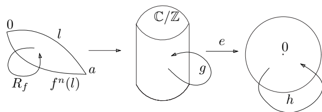
FIGURE 1. Schematics of cylinder renormalization.
