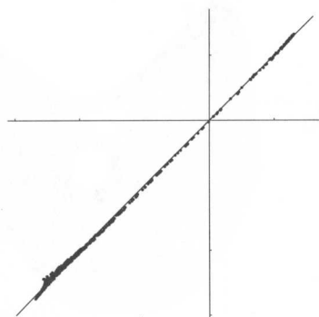
FIGURE 15. Plot of \frac{1}{\sqrt{C}} x \cdot n versus H\sqrt{C} for the octahedron.
