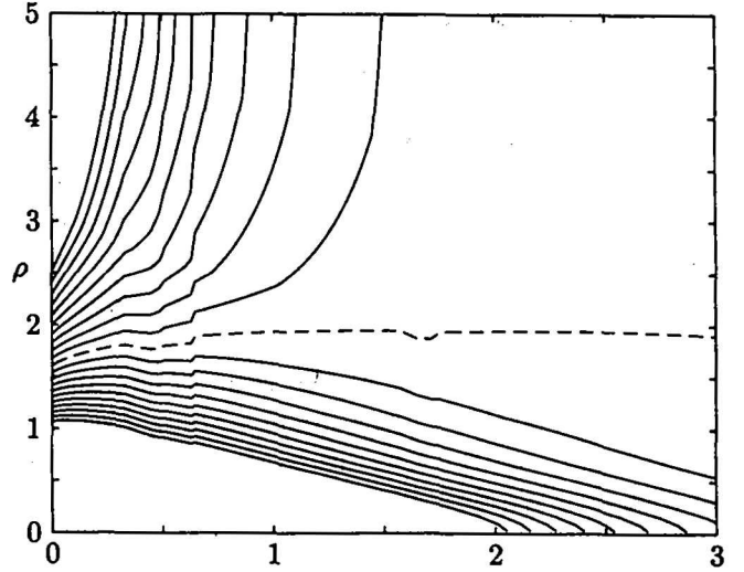
FIGURE 5. Trajectories of the level sets of \psi for the torus example, computed using the algorithm of Section 2.3 (compare Figure 4).
