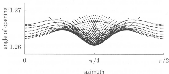
FIGURE 28. Angle of opening versus azimuth for the four-handled cone.
