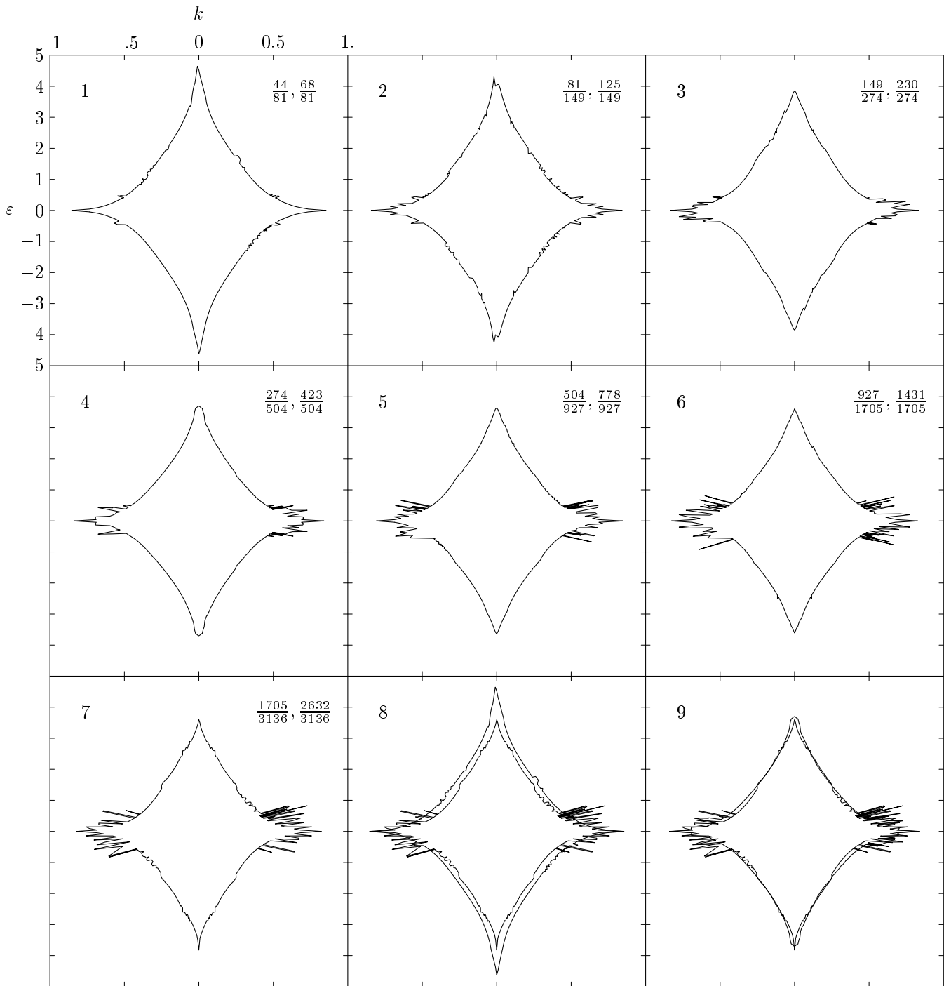
FIGURE 1. Domain of existence for the invariant surface with golden rotation vector (1, 1)^\infty , for real values of the parameters. Plots 1–7 represent the boundary where the residue of periodic orbits is 1, for the given values of the rotation vector, which were chosen as Jacobi–Perron convergents to (1, 1)^\infty . Plot 8 is a superimposition of 1 and 7, and 9 is a superimposition of 4 and 7. The ranges of k and \varepsilon are the same in all plots.
