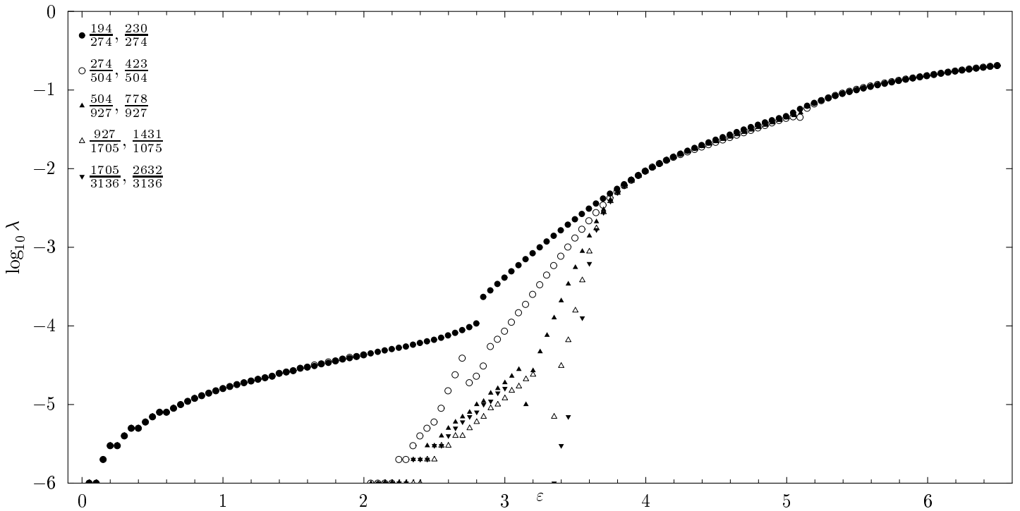
FIGURE 7. Stability index of the periodic orbits in the preceding figure. The jumps in the figure correspond to stability changes of the periodic orbit.
