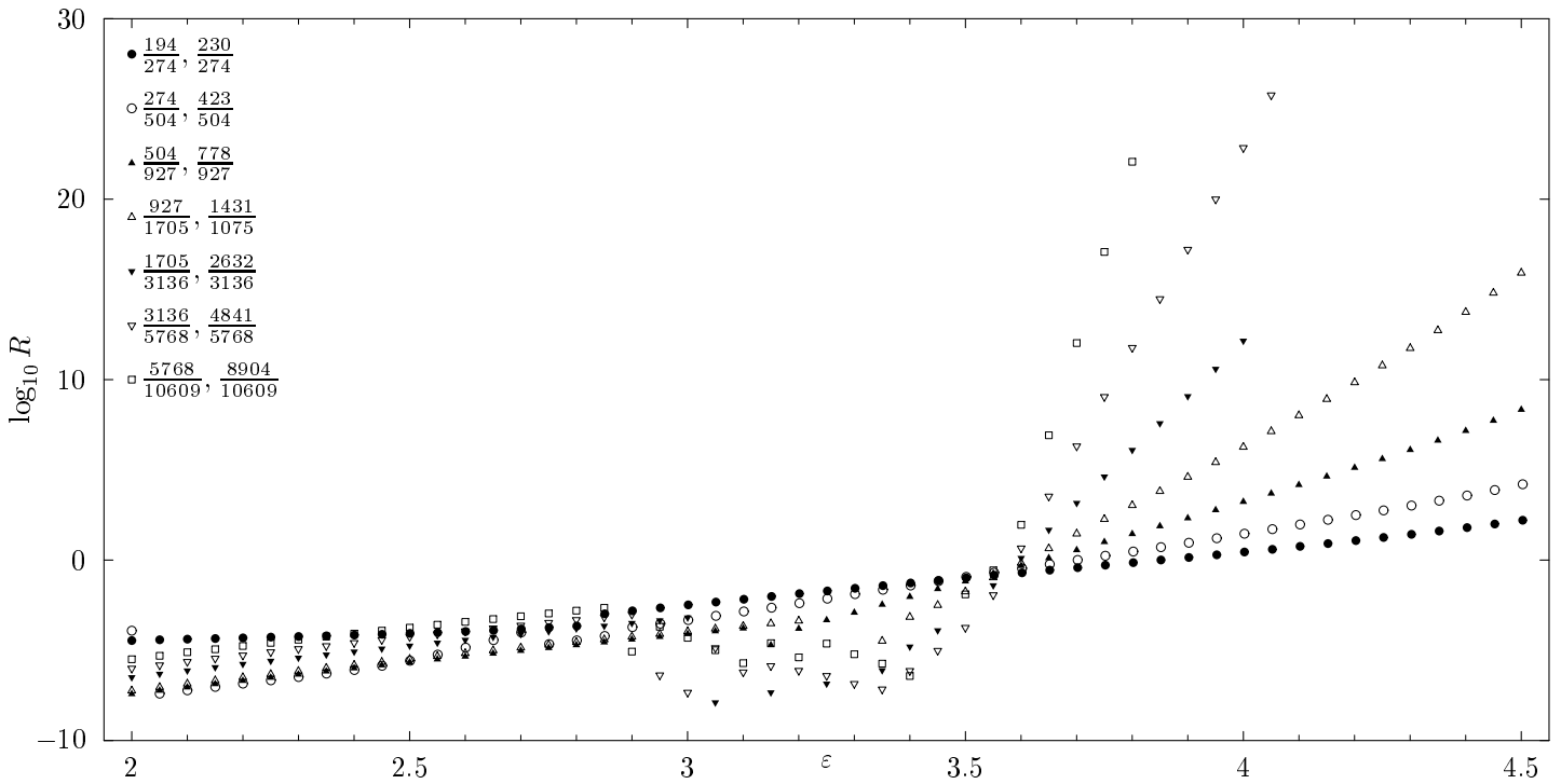
FIGURE 6. Residue of periodic orbits approximating an invariant set with rotation vector (1, 1)^\infty along the path k = 0 . The different sets correspond to different periodic orbits, with the ratios shown.
