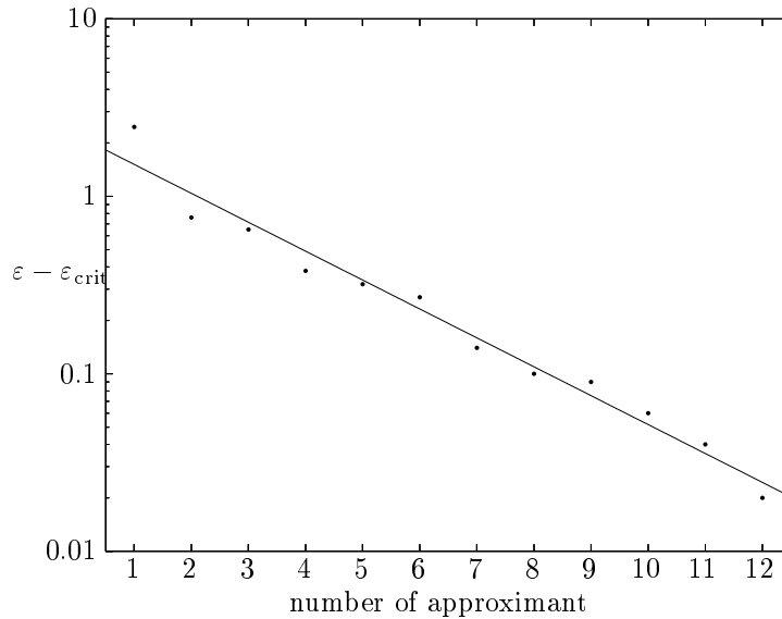
FIGURE 4. Scaling of the points where the residue becomes 1 for k = 0 , for successive Jacobi–Perron approximants to (1, 1)^\infty . The first approximant is (\frac{7}{13}, \frac{11}{13}) and the last is (\frac{5768}{10609}, \frac{8904}{10609}) . The value of \varepsilon_{\text{crit}} and the approximating straight line are determined from a least squares Levenberg–Marquardt scheme [Press et al. 1992]; the line has equation y = 2.2e^{-0.375x} .
