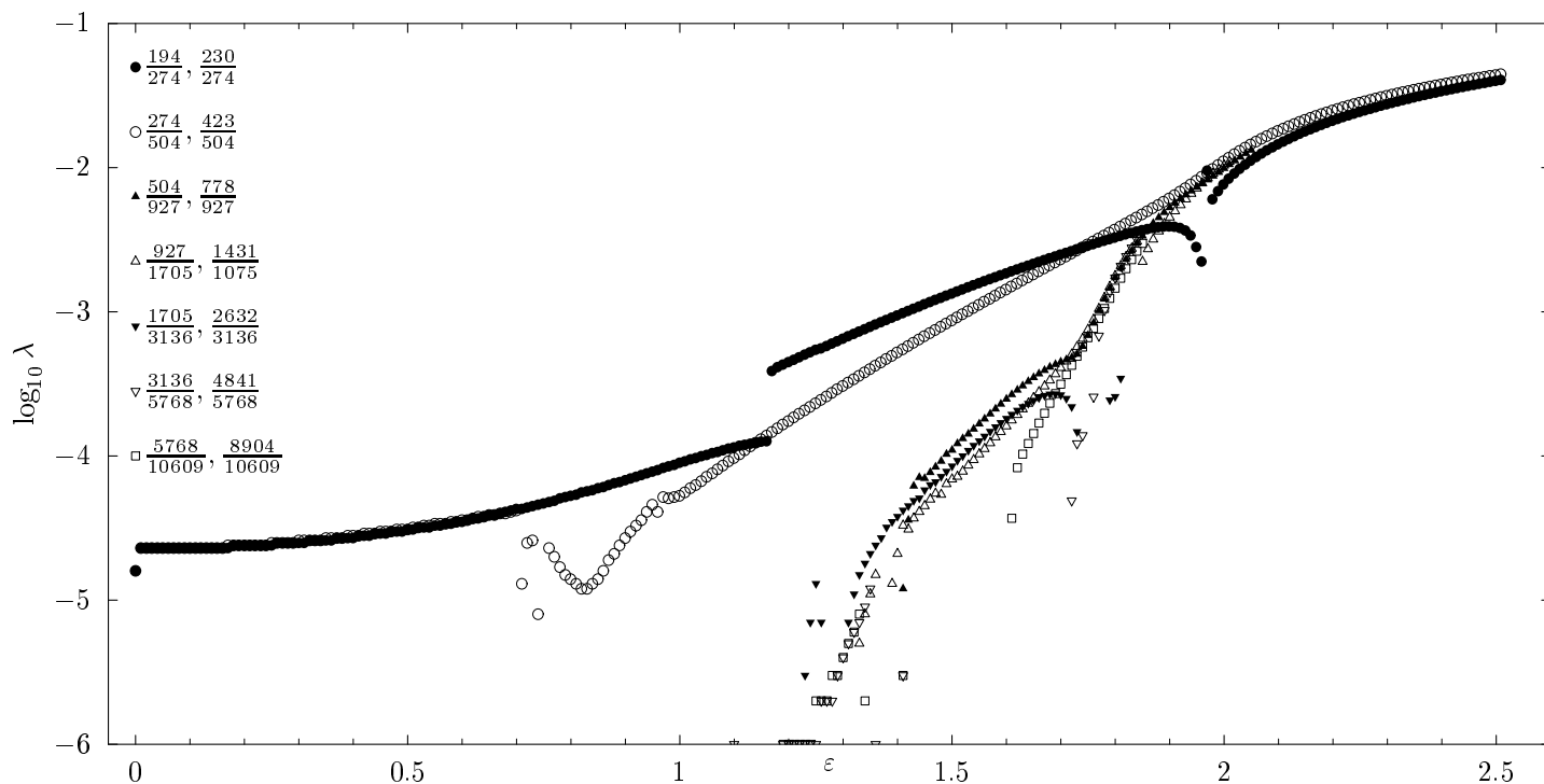
FIGURE 8. Stability index \lambda of periodic orbits approximating an invariant set with rotation vector (1,1)^\infty along the path k = 0.2 .
