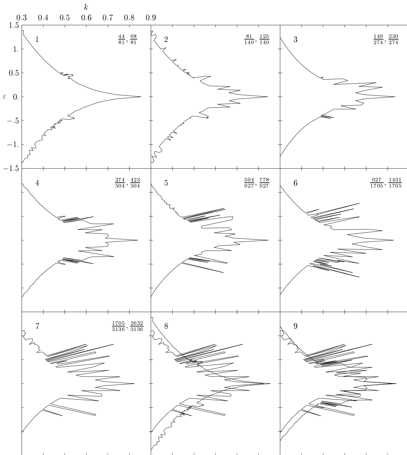
FIGURE 2. Detail of Figure 1.
