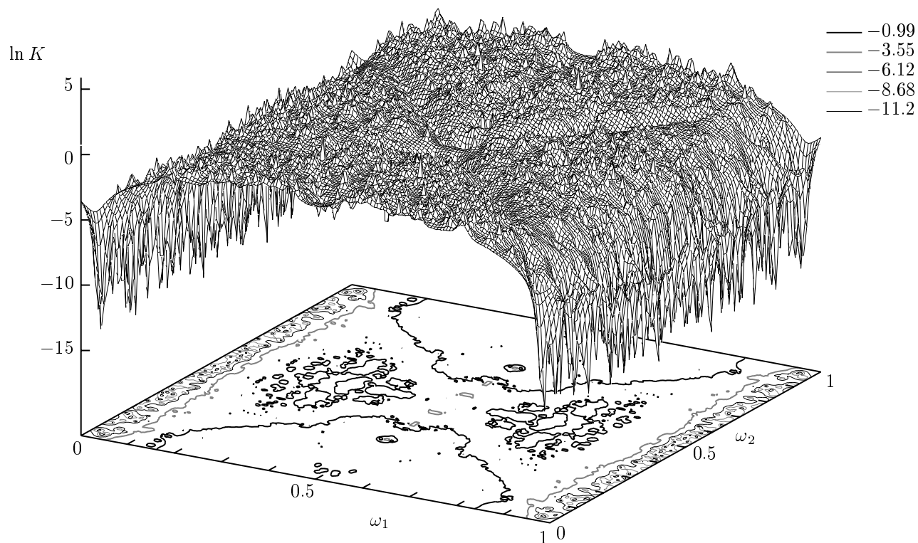
FIGURE 9. Logarithm of the critical function at k = 0.2 . The values of the function are computed using the residue of 6576 periodic orbits and interpolating on a 150 \times 150 grid. Some level sets are also drawn.
