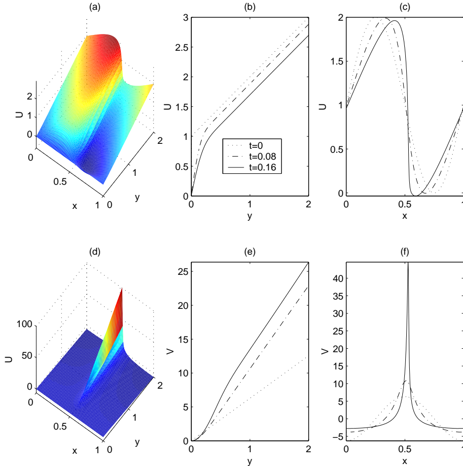
FIG. 4.3. A numerical solution of the viscous Prandtl equations (1.1) for \nu = 0.1 , with p^\infty = 0 , the initial data (3.9), and the boundary condition (4.13): (a) surface plot of u(x, y, t) at t = 0.16 ; (b) plots of u(x, y, t) versus y at x = 0.5 showing the formation of a boundary layer; (c) plots of u(x, y, t) versus x at y = 1 showing the formation of a shock; (d) surface plot of v(x, y, t) at t = 0.16 ; (e) plots of v(x, y, t) versus y at x = 0.5 ; (f) plots of v(x, y, t) versus x at y = 1 showing the formation of a singularity.
