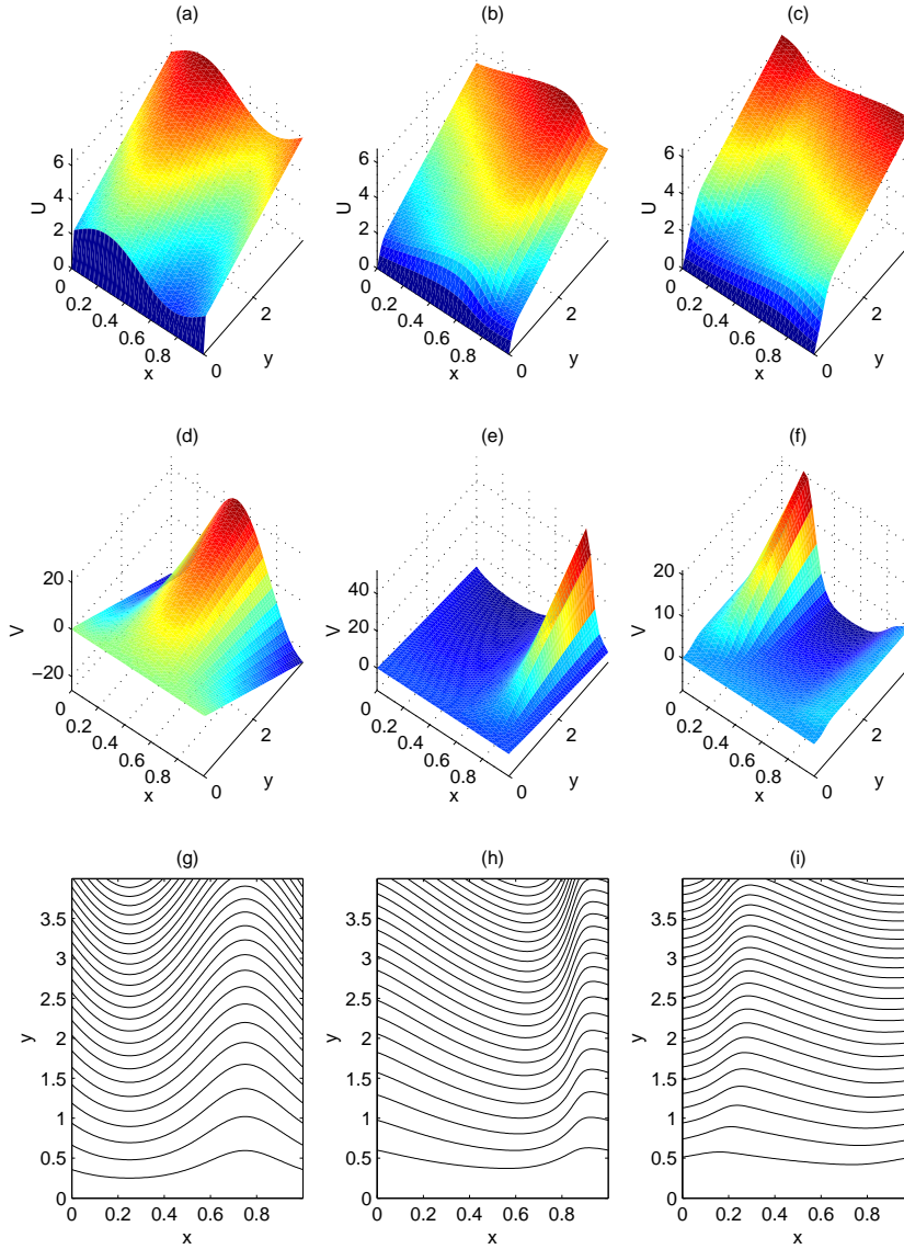
FIG. 4.1. A numerical solution of the viscous Prandtl equations (1.1) for \nu = 0.1 , with p^\infty = 0 , the initial data (4.12), and the boundary condition (4.13): (a)–(c) surface plots of u(x, y, t) at t = 0.0, 0.15, 0.3 ; (d)–(f) surface plots of v(x, y, t) at t = 0.0, 0.15, 0.3 ; (g)–(i) streamlines at t = 0.0, 0.15, 0.3 .
