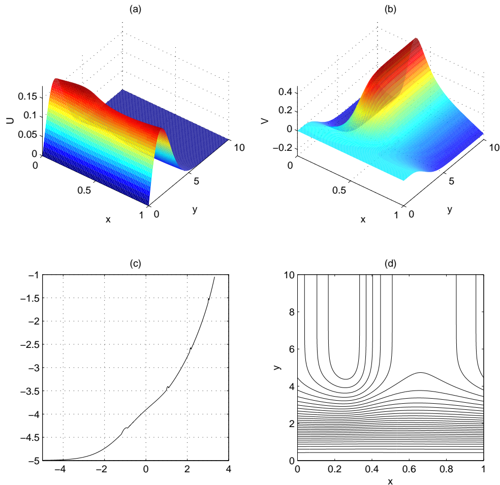
FIG. 6.2. A numerical solution of the viscous Prandtl equations (1.1), with u^\infty = 0 and the initial data u_0(x, y) = U(y)[1 + 0.005 \sin(2\pi x)] , where U(y) = 2ye^{-y^2} : (a) a surface plot of u(x, y, t) at time t = 10 ; (b) a surface plot of v(x, y, t) at time t = 10 ; (c) a log-log plot of the maximum norm \|v\|_\infty of v versus t ; (d) streamlines at t = 10 .
