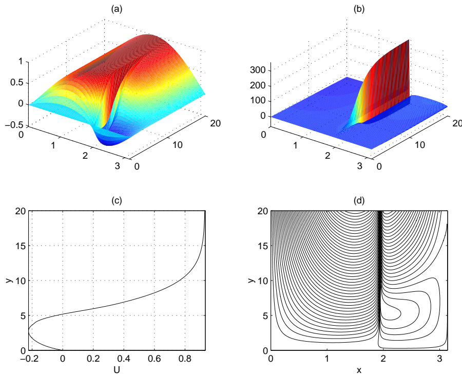
FIG. 4.4. A numerical solution of the viscous Prandtl equations (1.1) with data (4.14), corresponding to flow past a cylinder started impulsively from rest at the singularity formation time t = 3.0 : (a) surface plot of u(x, y, t) ; (b) surface plot of v(x, y, t) ; (c) profile of u versus y at x = 1.94 ; (d) streamlines.
