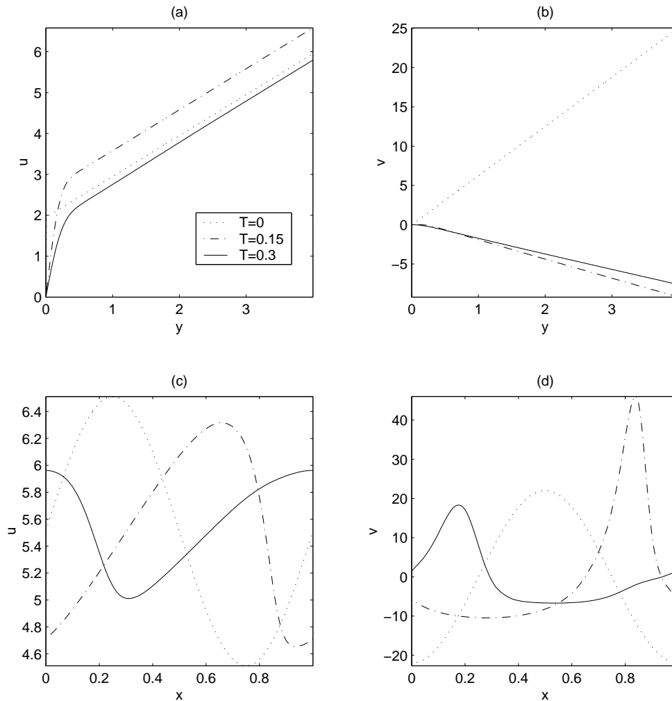
FIG. 4.2. Plots of u and v for the numerical solution of the viscous Prandtl equations shown in Figure 4.1: (a) u(x, y, t) versus y at x = 0.5 ; (b) v(x, y, t) versus y at x = 0.5 ; (c) u(x, y, t) versus x at y = 3.5 ; (d) v(x, y, t) versus x at y = 3.5 .
