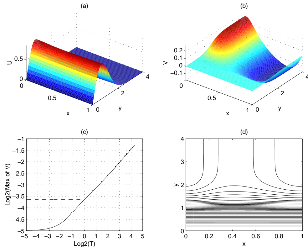
FIG. 6.1. A numerical solution of the inviscid Prandtl equations (2.1)–(2.4), with the initial data u_0(x, y) = U(y) [1 + 0.005 \sin(2\pi x)] , where U(y) = 2ye^{-y^2} : (a) a surface plot of u(x, y, t) at time t = 10 ; (b) a surface plot of v(x, y, t) at time t = 10 ; (c) a log-log plot of the maximum norm \|v\|_\infty of v versus t ; (d) streamlines at t = 10 .
