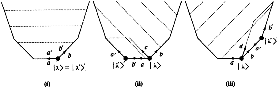
Fig. 2. Spectral Flow for the \mathcal{S}'\mathcal{W}_{1+\infty} Algebra
