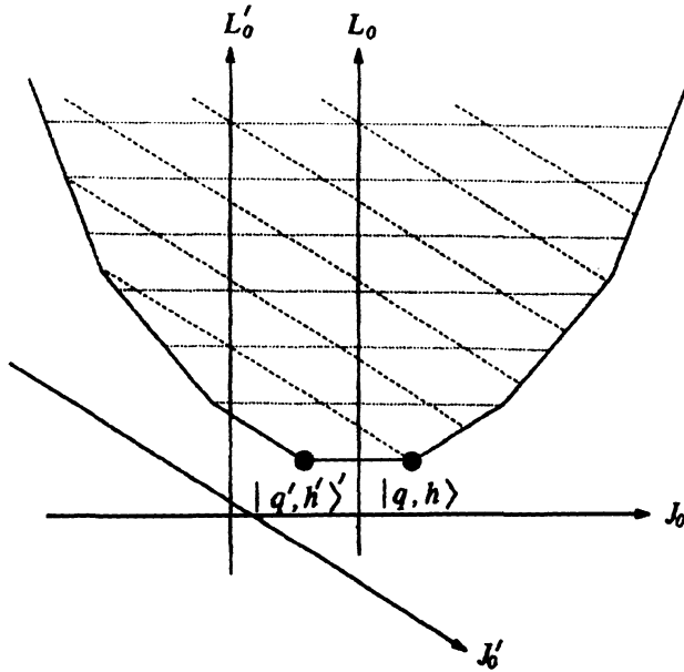
Fig. 1. Spectral Flow for the N = 2 Superconformal Algebra
