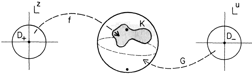
Fig. 1. Defining $G$ from $f$
