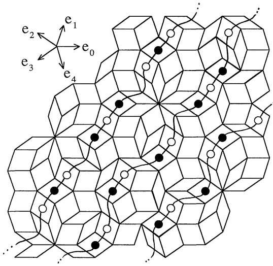
Fig. 2. Definition of the alternation condition. The star vectors are shown in the inset. (2, 3)-tiles are marked with a solid circle. (2, 1)-tiles are marked with an open circle. Along every 2-row the solid and open circles alternate. Note that the (2, 0) and (2, 4) tiles alternate also. The curvy lines are guides to the eye that follow the 2-rows
