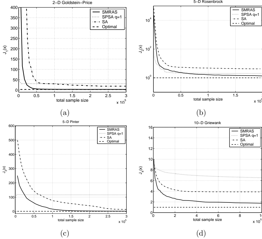
FIG. 3. Performance of SMRAS, SPSA, and SA on (a) Goldstein-price function; (b) 5-D Rosenbrock function; (c) 5-D Pinter function; (d) 10-D Griewank function.
