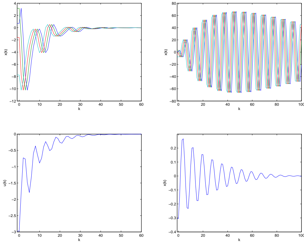
FIG. 4. Example 1. State responses and control input under state feedback law: r = 1 and \varepsilon = 0.2 (left plots); r = 1 and \varepsilon = 0.02 (right plots).
