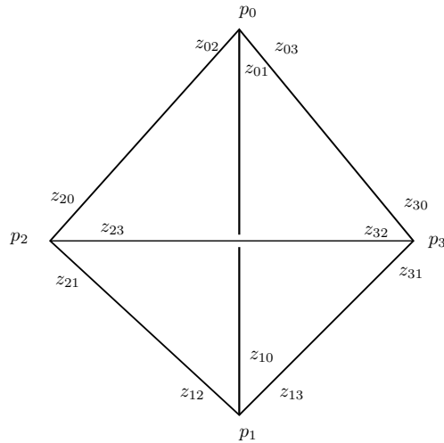
FIG. 1. Parameters for a cross-ratio structure
