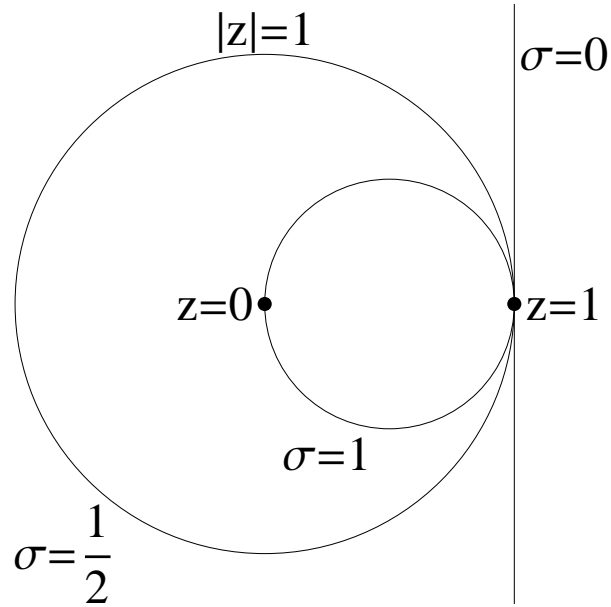
FIGURE 4. z-plane
