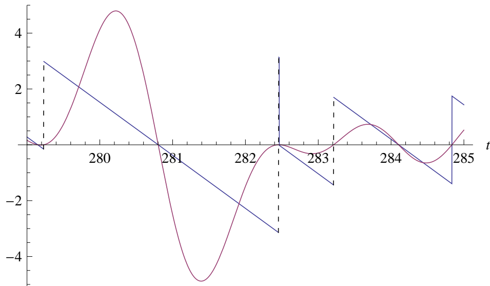
FIGURE 2. Plot of \text{Im } \zeta \left( \frac{1}{2} + it \right) (continuous curve) and \text{Im } \ln \left( \zeta \left( \frac{1}{2} + it \right) \right) = \pi S(t) (step curve).
