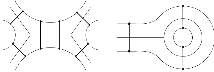
Figure 5. Cellular decomposition via fatgraphs.
