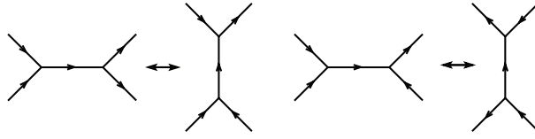
Figure 2. Flip transformation for oriented fatgraphs.
