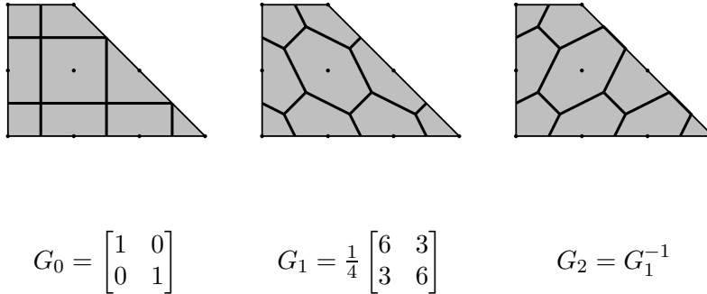
Figure 7. GQ amoebas associated to different quadratic \psi 's.
