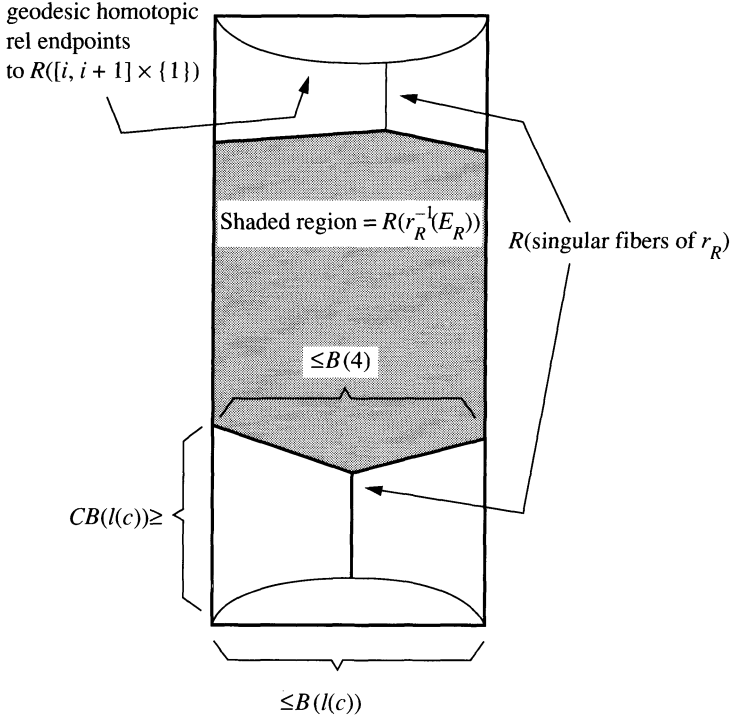
FIGURE 4. R([i, i + 1] \times I) = \Delta Q_V([i, i + 1] \times I) .
