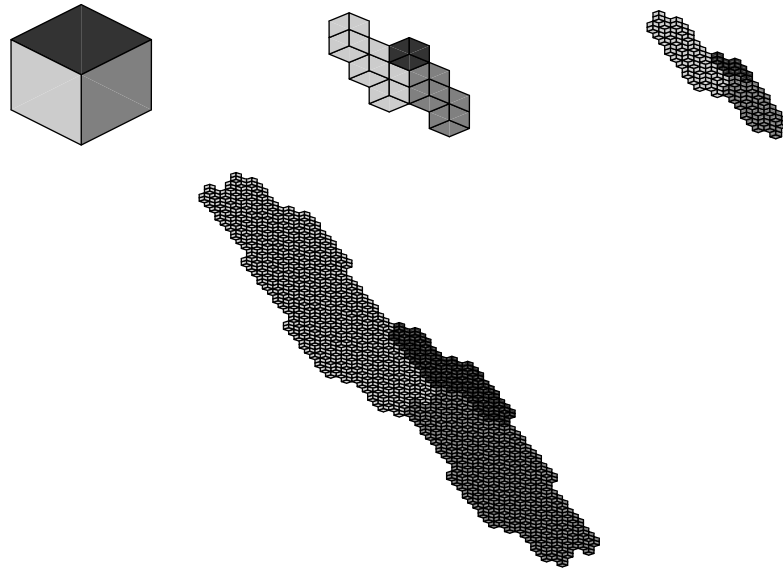
Figure 11: The figure of E_1^*(\sigma)^n(0, e_1^*) for \sigma = \sigma_1\sigma_2^2\sigma_3 , \mathbf{i} = \mathbf{1}, \mathbf{2}, \mathbf{3} , n = 0, 1, 2, 3
