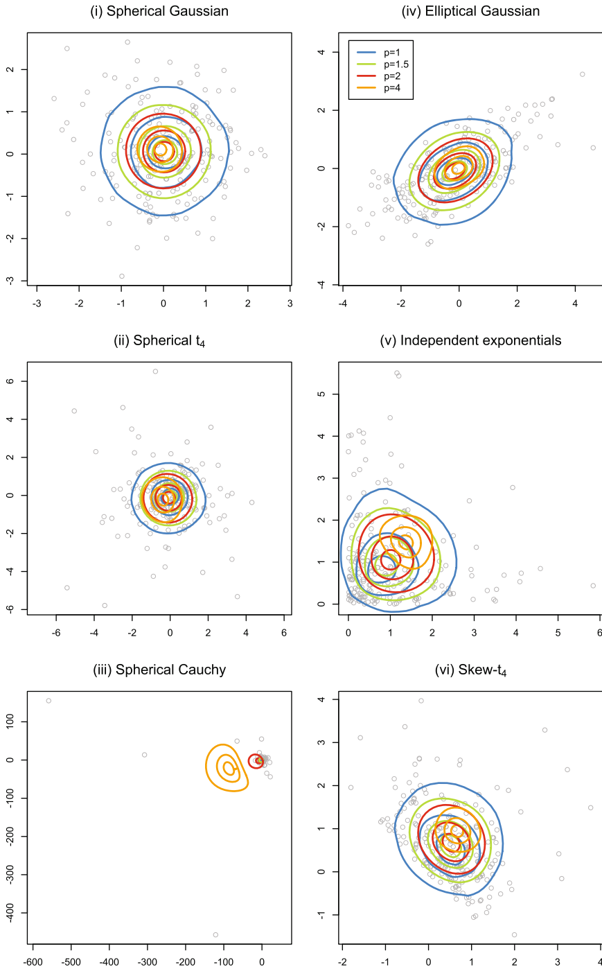
Figure 2. For \rho(t) = t^p with p = 1, 1.5, 2, 4 , \rho -depth contours of order \alpha = .25, .50, .75 for random samples of size n = 200 drawn from six bivariate distributions; see Section 6 for details.
