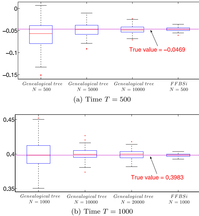
Figure 2. Computation of smoothed additive functionals in a linear Gaussian model. The variance of the estimation given by the FFBSi algorithm is the smallest one in both cases.
