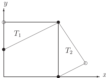
FIGURE 1. Triangles that disappear.
