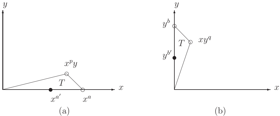
FIGURE 2. Case where a vertex x^p y^q of \Gamma(f_s) disappears: (a) q = 1 ; (b) p = 1 .
