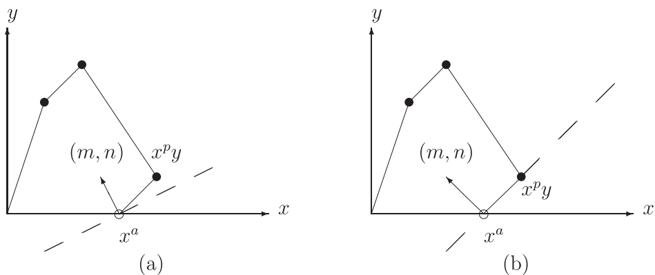
FIGURE 5. Case where a monomial x^a of \Gamma(f_s) disappears: (a) \gamma = \{x^a\} ; (b) \gamma joints the vertices x^a and x^p y .
