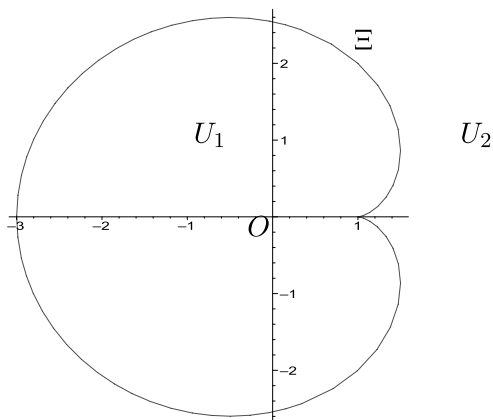
FIGURE 3. Degeneration locus \Xi
