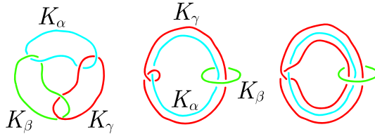
Figure 3. (left, center) \mathcal{C}_3 . (right) \bar{b} . (This figure explains how to obtain H .)
