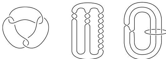
Figure 1. (left) 3 chain link C_3 . (center) (-2, 3, 8) -pretzel link or Whitehead sister link. (right) link 6_2^2 .
