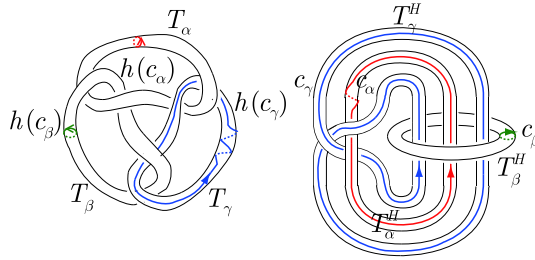
Figure 5. (left) h(c_\alpha), h(c_\beta), h(c_\gamma) . (right) c_\alpha, c_\beta, c_\gamma .
