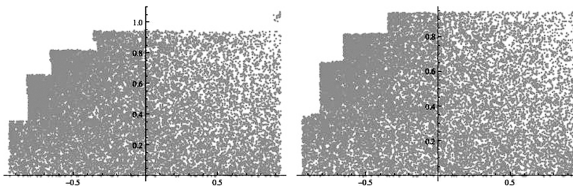
Figure 8. Change of topology at \alpha = \alpha_0 : Simulations of the natural extension for q = 9 ; on left \alpha = \alpha_0 - 0.001 , on right \alpha = \alpha_0 + 0.001 .
