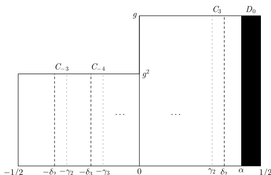
Figure 2. Regions of change of digit and basic deletion. Here each \gamma_m represents \delta_m(1/2) . To aid visualization, we use here C_{\varepsilon r} = C \cap \Delta(\varepsilon : r) . Note that C = \bigcup_{\{\varepsilon, r\}} C_{\varepsilon, r} .
