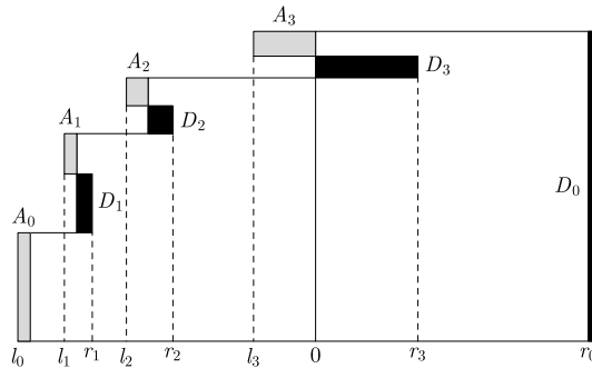
Figure 5. The added and deleted rectangles for \alpha = 0.48 in the natural extensions for q = 8 . Here A_i, D_i denote \mathcal{T}^i(A_0), \mathcal{T}^i(D_0) , respectively.
