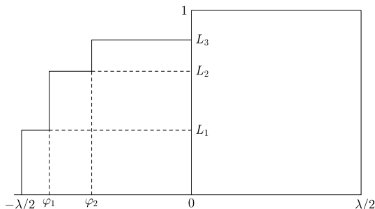
Figure 7. The natural extension for q = 7 and \alpha = 1/2 .
