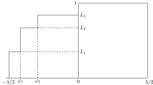
Figure 4. The natural extension for q = 8 and \alpha = 1/2 .
