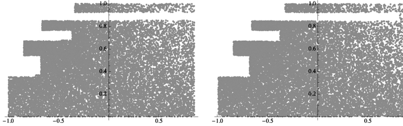
Figure 6. Change of topology at \alpha = \alpha_0 : Simulations of the natural extension for q = 8 with on the left \alpha = \alpha_0 - 0.001 and on the right \alpha = \alpha_0 + 0.001 .
