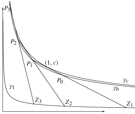
FIGURE 1. Special points P_0 = (w_+, v_+) , P_1 = (w_-, v_-) , P_2, \dots and Z_1 = (z, z^{1/(1-p)}) , Z_2, Z_3, \dots
