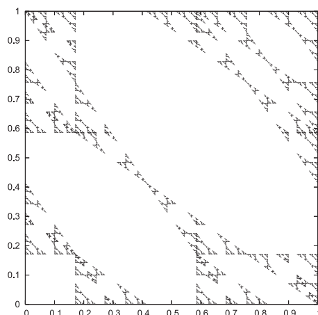
Figure 5.4. Aperiodic points, \lambda = -\sqrt{2} .
