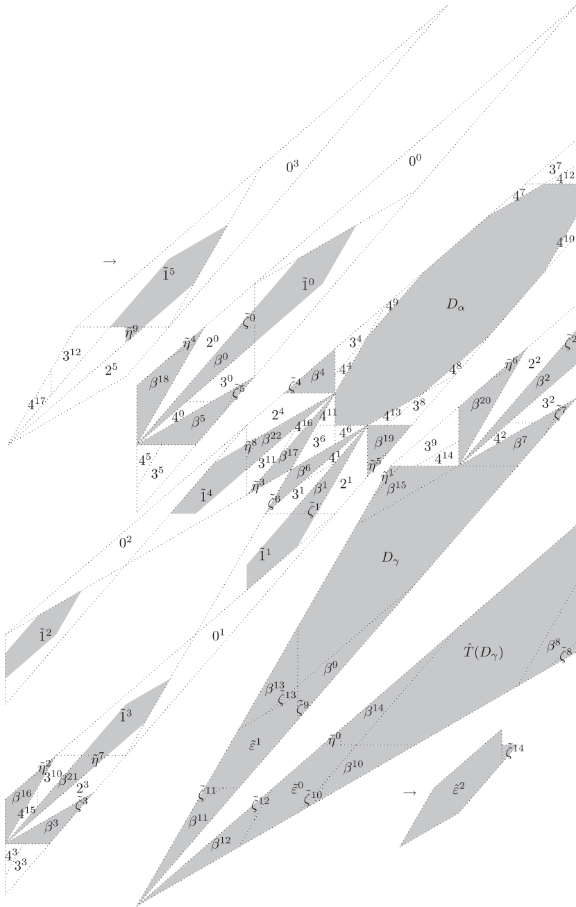
Figure 9.2. The trajectory of the open scaled sets in \mathcal{D}_1 and the set \mathcal{P}_1 , \lambda = \sqrt{3} . ( \ell^k stands for \hat{T}^k U_1(D_\ell) if \ell \in \{0, 1, 2, 3, 4\} , for \hat{T}^k(D_\ell) else.)
