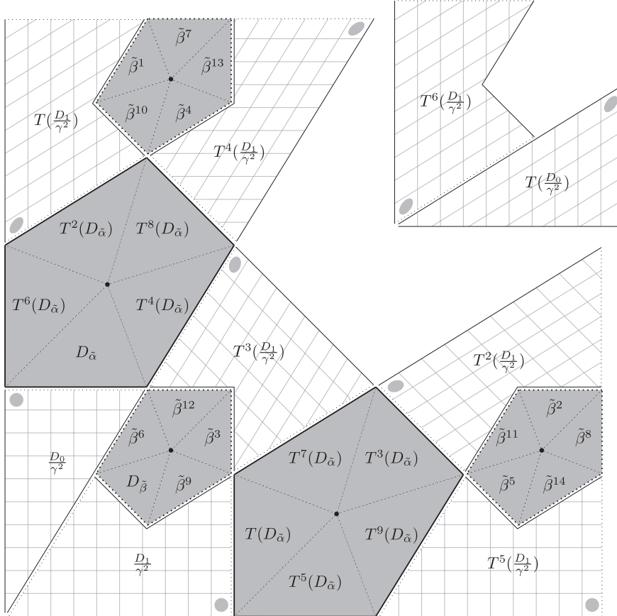
Figure 2.2. The trajectory of the scaled domains and the (gray) set \mathcal{P} , \lambda = \gamma . ( \tilde{\beta}^k stands for T^k(D_{\hat{\beta}}) .)
