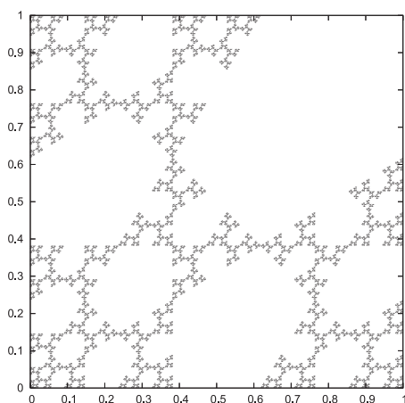
Figure 2.3. Aperiodic points, \lambda = \gamma .
