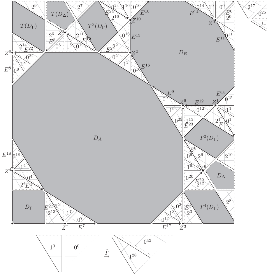
Figure 8.1. The map \hat{T} and the set \mathcal{R} , \lambda = -\gamma . ( \ell^k stands for T^k(D_\Gamma) .)
