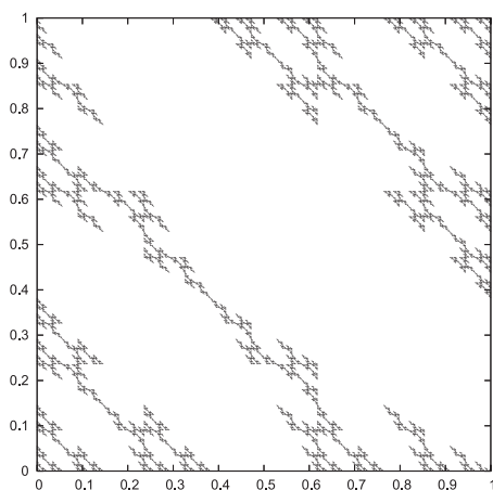
Figure 2.4. Aperiodic points, \lambda = -1/\gamma .
