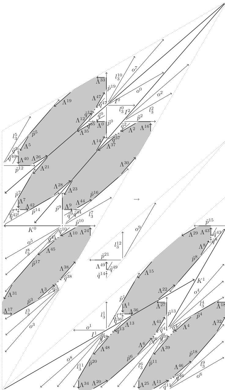
Figure A.4. The trajectory of the lines, \lambda = \sqrt{3} . ( l^k stands for \tilde{T}_3^k(D_l) .)
