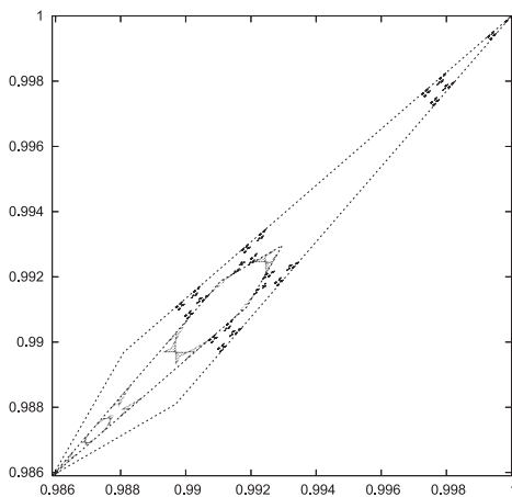
Figure 9.7. Aperiodic points in \mathcal{D}_1 \cup \mathcal{D}_2 , \lambda = \sqrt{3} .
