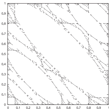
Figure 10.4. Aperiodic points, \lambda = -\sqrt{3} .
