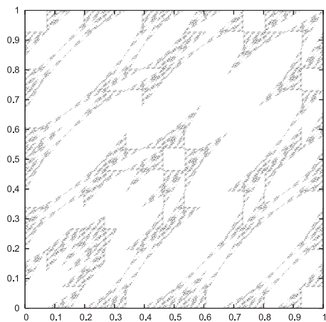
Figure 9.6. Aperiodic points, \lambda = \sqrt{3} .
