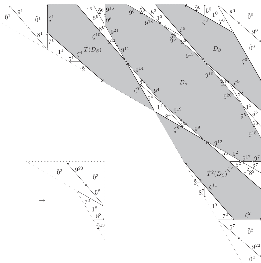
Figure 10.2. Trajectory of U_1(\mathcal{P}) and large parts of \mathcal{P} , \lambda = -\sqrt{3} . ( \ell^k stands for \hat{T}^k U_1(D_\ell) .)
