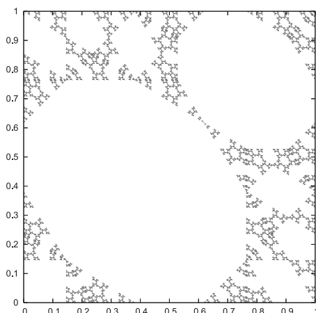
Figure 7.4. Aperiodic points, \lambda = -\gamma .
