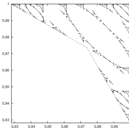
Figure 10.5. Aperiodic points in \mathcal{Q} , \lambda = -\sqrt{3} .
