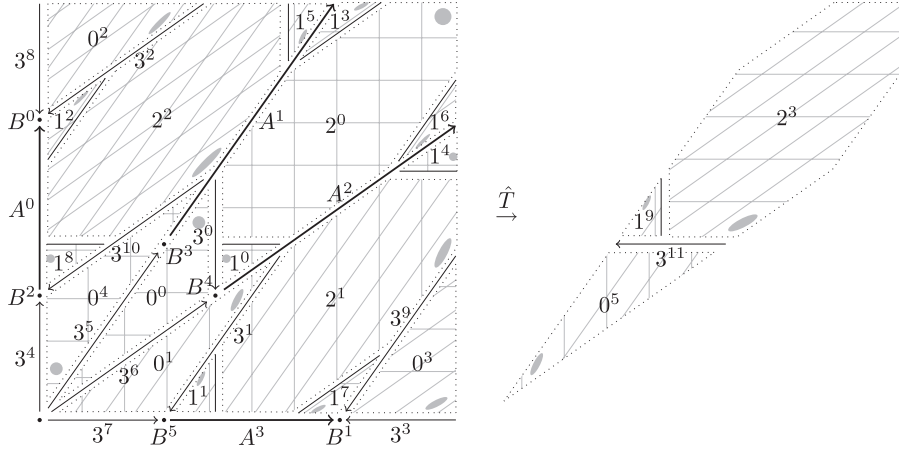
Figure 5.1. The map \hat{T} and the set \mathcal{A} , \lambda = \sqrt{2} . ( \ell^k stands for T^k(D_\ell) .)
