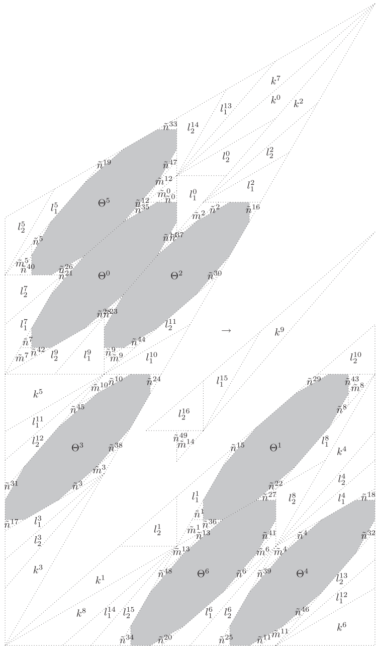
Figure A.3. An intermediate first return map, \lambda = \sqrt{3} . ( \ell^k stands for \hat{T}_3^k(D_\rho) .)
