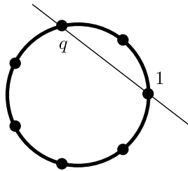
Figure 3 For m = 7 , the group \mathbb{G}(\mathbb{R}) = \text{SU}(h, h + 5) \times \text{SU}(h + 1, h + 4) \times \text{SU}(h + 2, h + 3)
