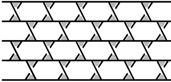
Figure 2 Schematic of a genus-6 surface with five boundary components and an action of \mathbb{Z}/5\mathbb{Z}
