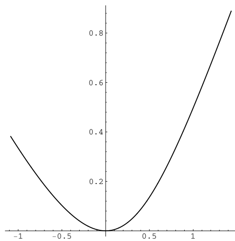
FIGURE 2c. \kappa(s) = \exp(s) in \mathbf{L}^2 .
