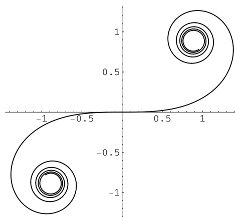
FIGURE 2b. Cornu spiral in \mathbf{R}^2 .
