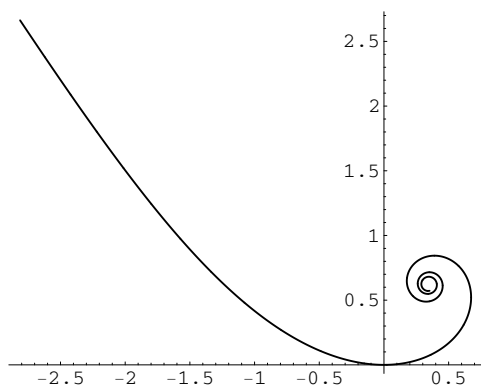
FIGURE 2d. \kappa(s) = \exp(s) in \mathbf{R}^2 .
