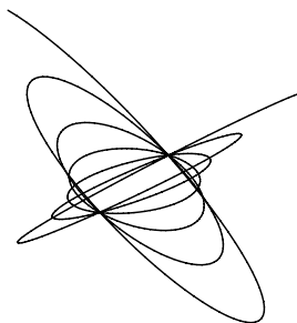
FIGURE 1b. \kappa(s) = \cos(s) .
