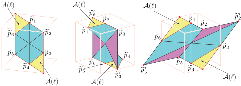
FIGURE 4. Coamoeba and zonotope chains.
