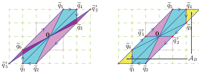
FIGURE 6. Images of \text{Arg}(\beta)(Z(\ell_B)) .
