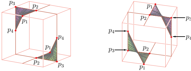
FIGURE 2. Two views of \mathcal{A}(\ell) .
