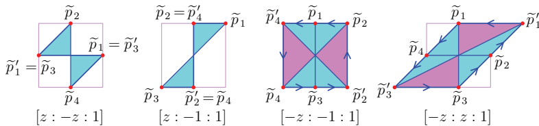
FIGURE 5. Four more zonotope chains.
