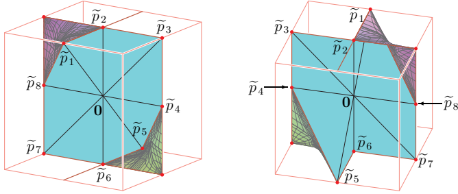
FIGURE 3. Two views of the coamoeba and zonotope chains.
