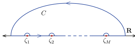
FIGURE 1. Contour in upper half plane.
