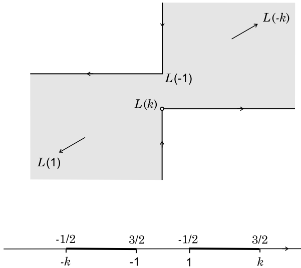
FIGURE 5. Limit of rescaled maps for k = k_{\text{crit}} .
