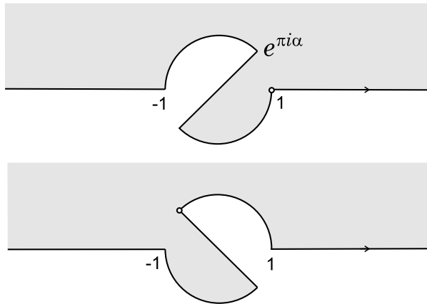
FIGURE 1. Two families of quadrilaterals.
