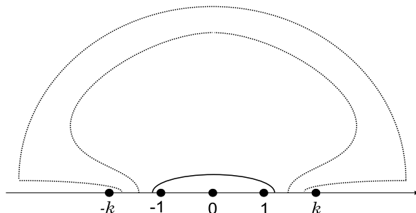
FIGURE 3. Deformation of the path of integration.
