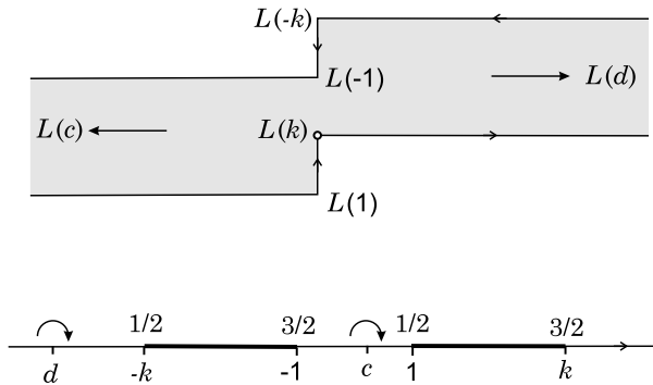
FIGURE 2. Conformal map, L = \log f .
