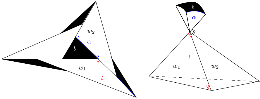
FIGURE 3. White faces around a black face define a convex cone.
