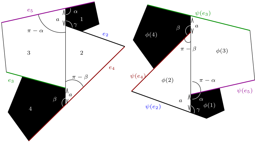
FIGURE 2. The “flip” of an edge.
