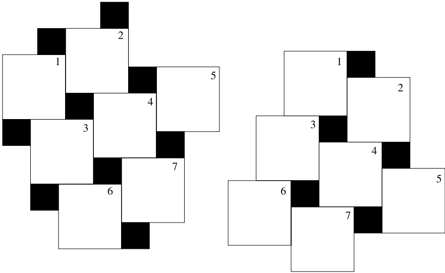
FIGURE 1. A flippable tiling, sometimes found in bathrooms—left and right versions.
