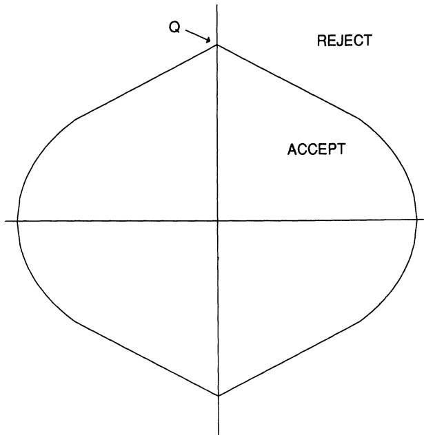
FIG. 2. The acceptance region of the L.R.T. when \sigma_1^2 = 2 and \sigma_2^2 = 1 .
