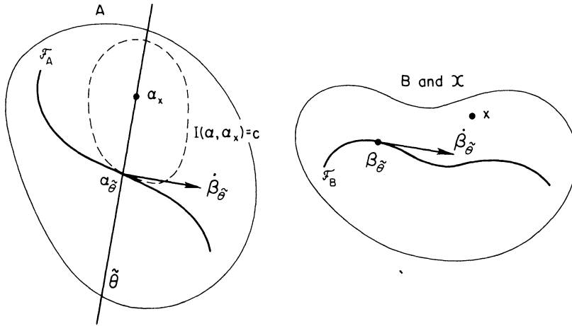
FIG. 6. A theory of estimation dual to maximum likelihood. This picture should be compared with Figure 1. The estimate \alpha_{\tilde{\theta}} is the projection of \alpha_x onto \mathcal{F}_A , orthogonally to \dot{\beta}_{\tilde{\theta}} . It is also the nearest point \alpha to \alpha_x on \mathcal{F}_A , measured in terms of I(\alpha, \alpha_x) .
